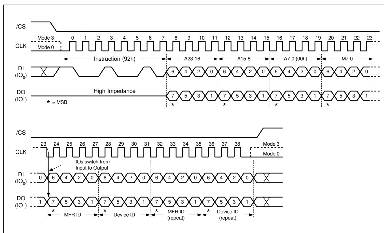
Figure 47. Read Manufacturer / Device ID Dual I/O Instruction
